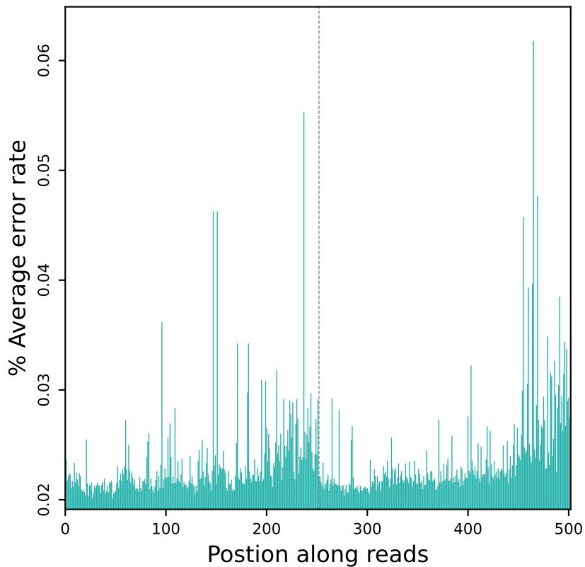
Error rate distribution along reads (R10425)
